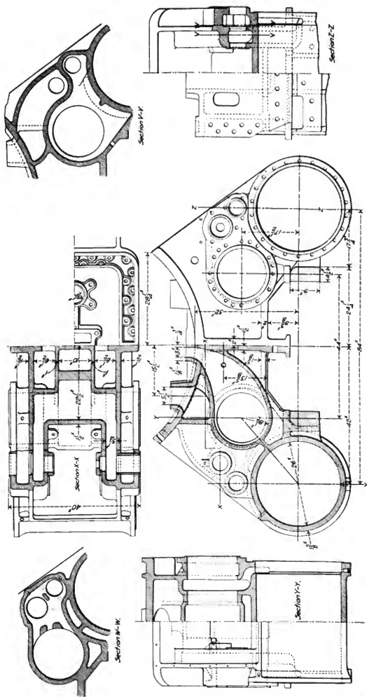
Figs. 861-866. Low Pressure Cylinders for Schenectady Tankem Compound Locomotive, Diameter 26 in. American Locomotive Co.
